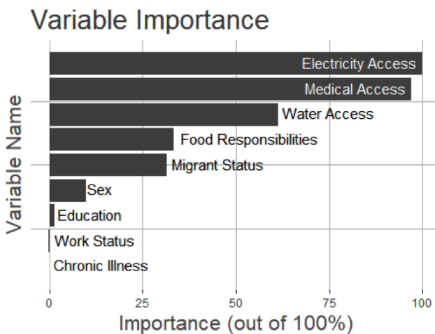
FIGURE 2: Support Vector Machine Variable Importance Calculations
